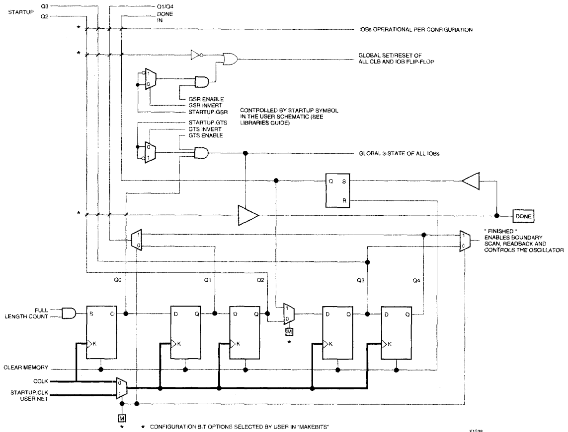
Figure 49: Start-up Logic
