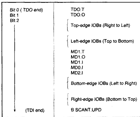
Figure 43: Boundary Scan Bit Sequence
