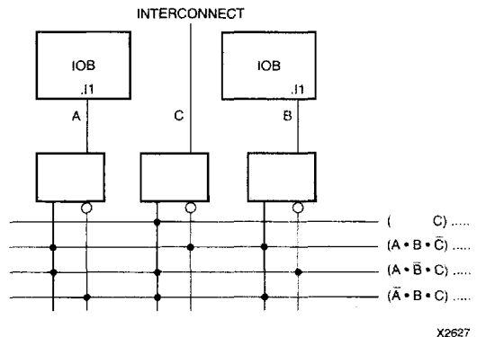
Figure 24: XC4000 Series Edge Decoding Example
