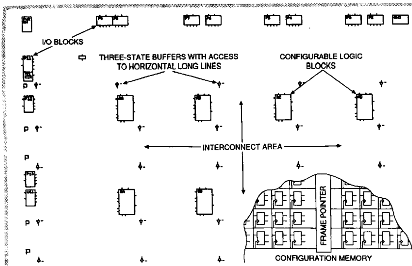
Figure 1. Field-Programmable Gate Array Structure
