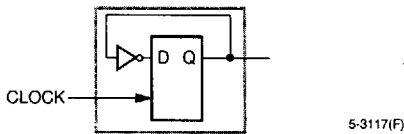
Figure 26. Toggle Flip-Flop
