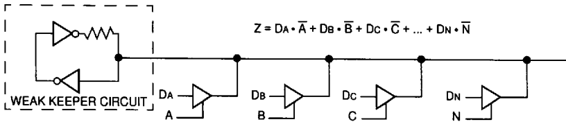
Figure 15B. 3-State Buffers Implement a Multiplexer
