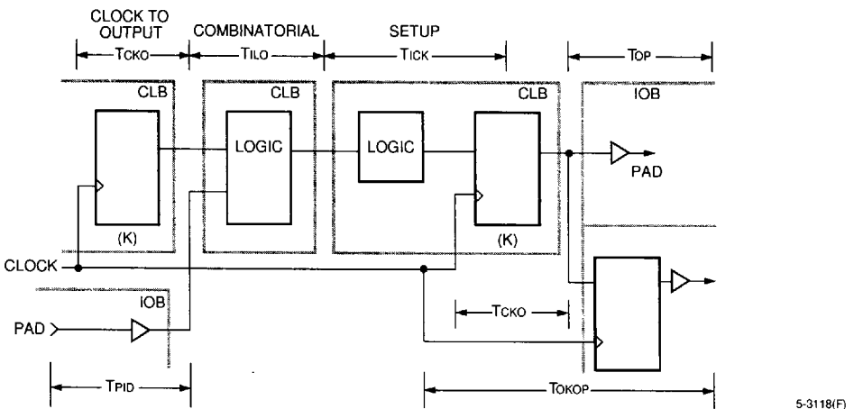
Figure 27. Examples of Primary Block Speed Factors
