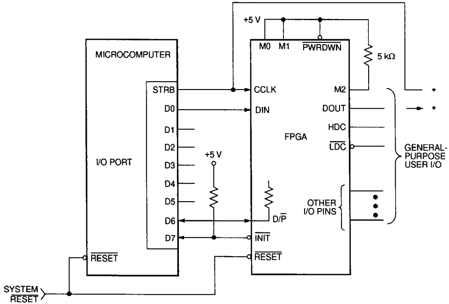
Figure 24. Slave Mode
