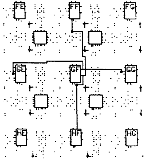
Figure 11. Direct Interconnect
