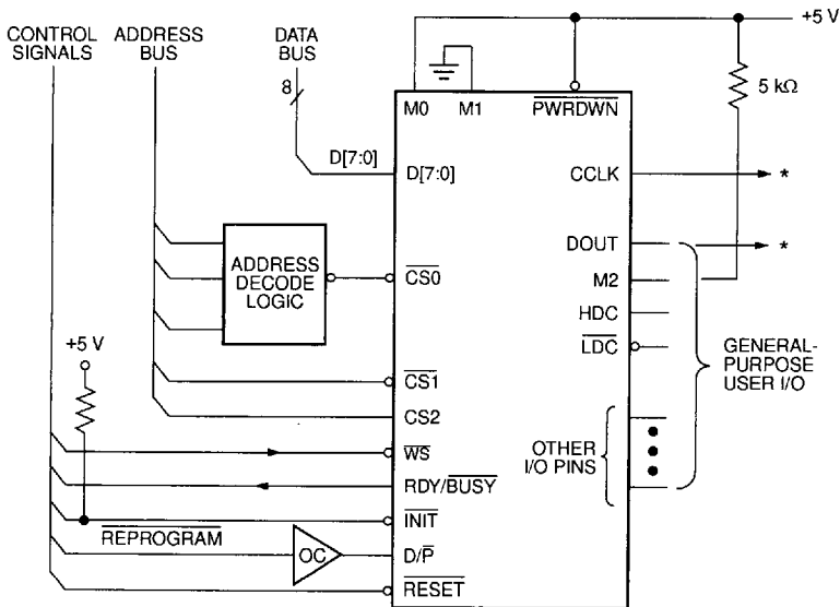
Figure 23. Peripheral Mode
