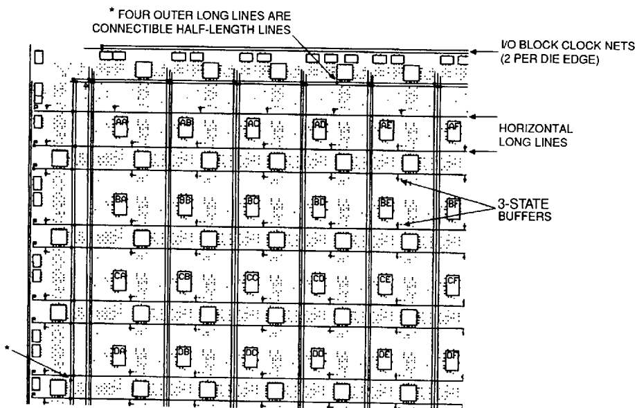
Figure 14. Programmable Interconnection of Long Lines
