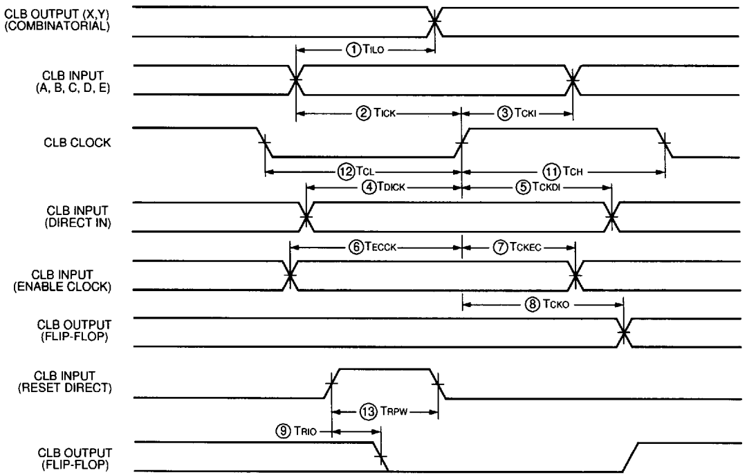
Figure 33. CLB Switching Characteristics
