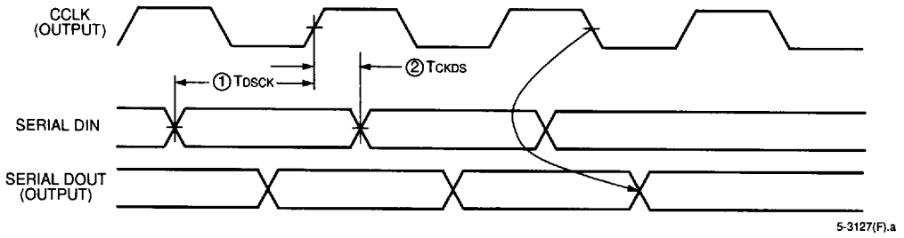
Figure 36. Master Serial Mode Switching Characteristics
