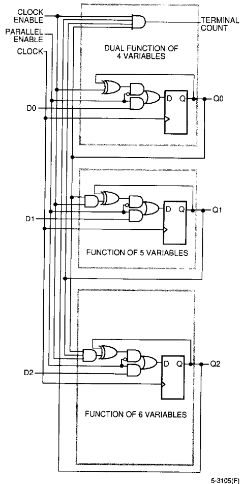
Figure 6. C8BCP Macro
