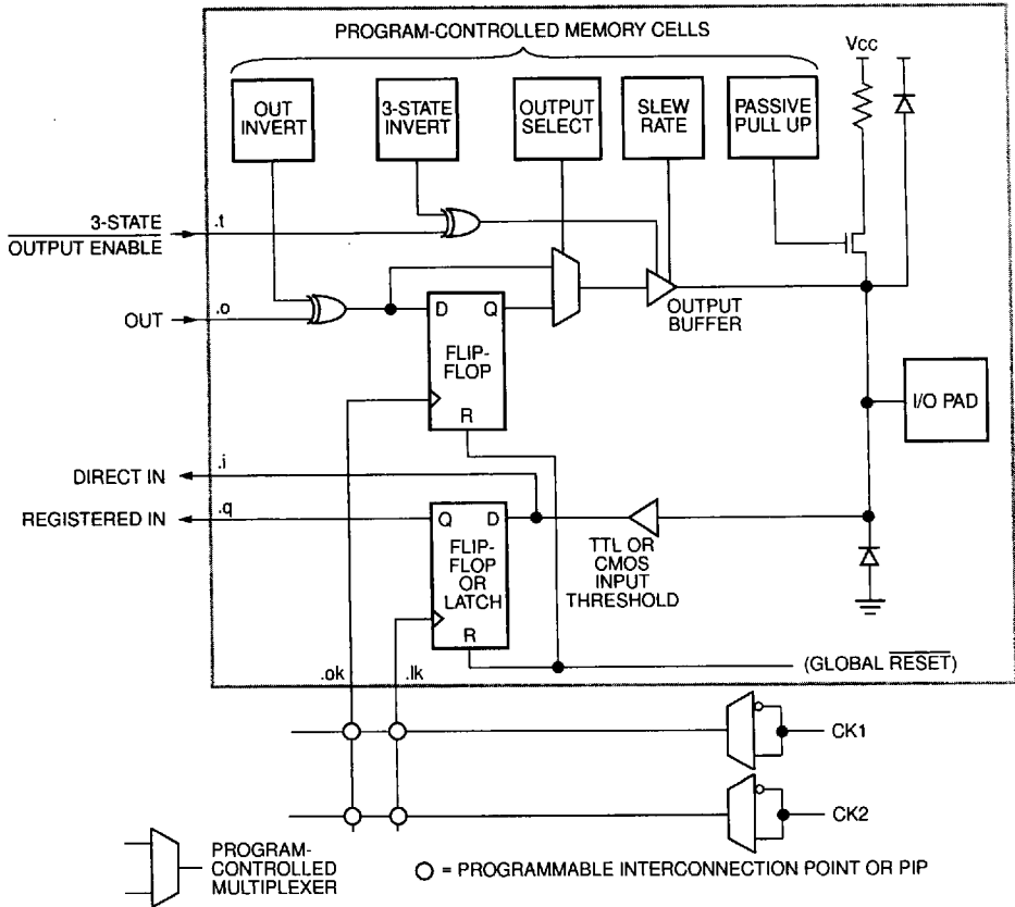
Figure 3. Input/Output Block
