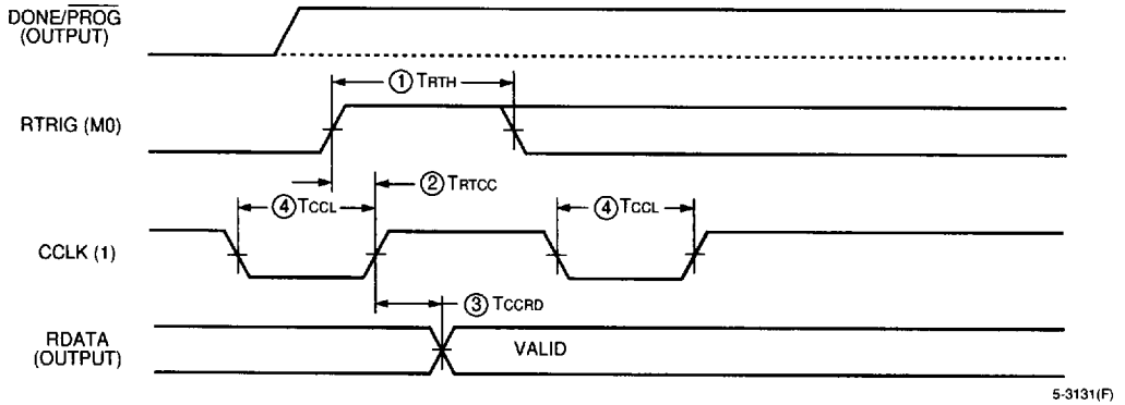
Figure 40. Program Readback Switching Characteristics
